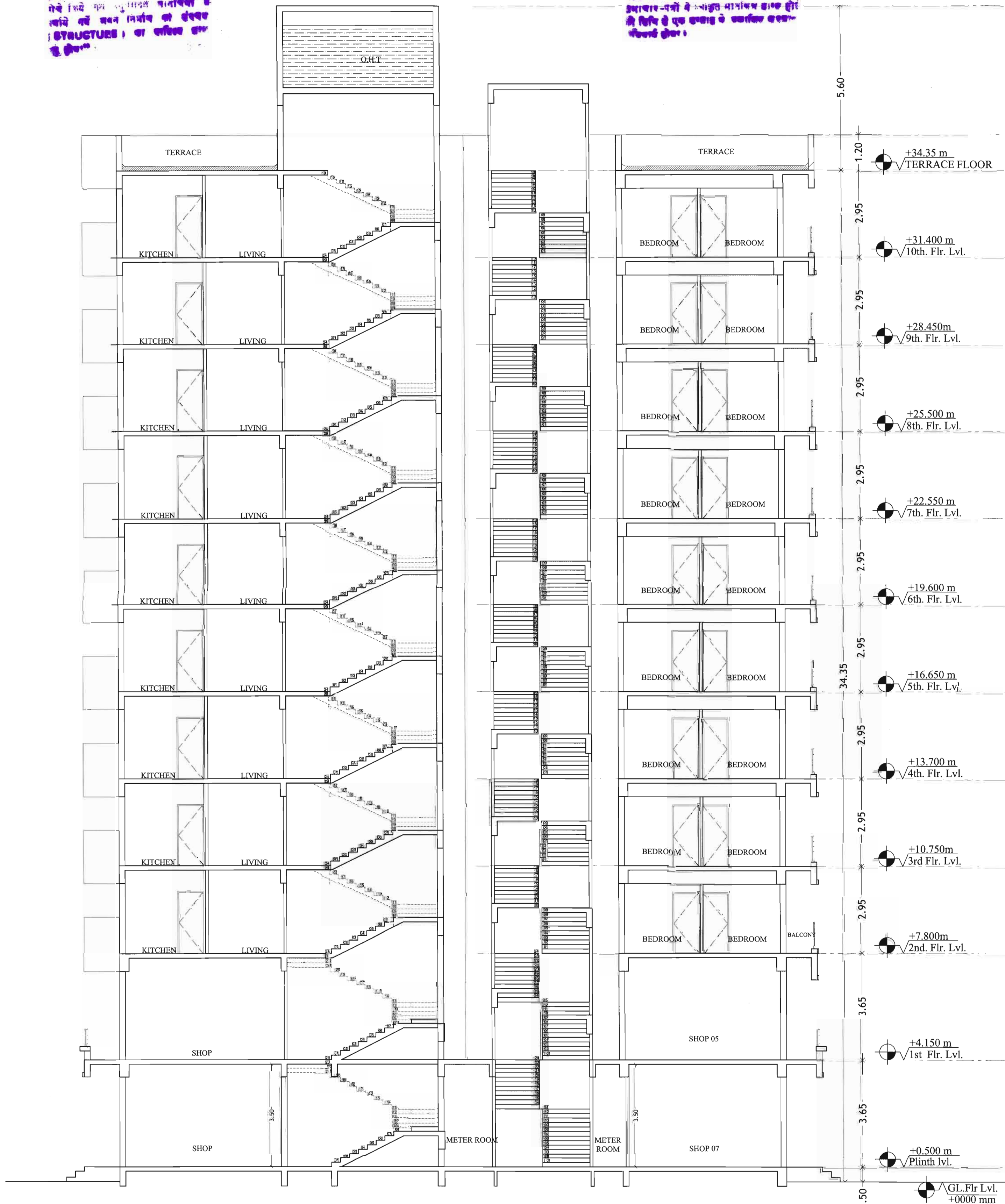
SECTION ON -01-01
