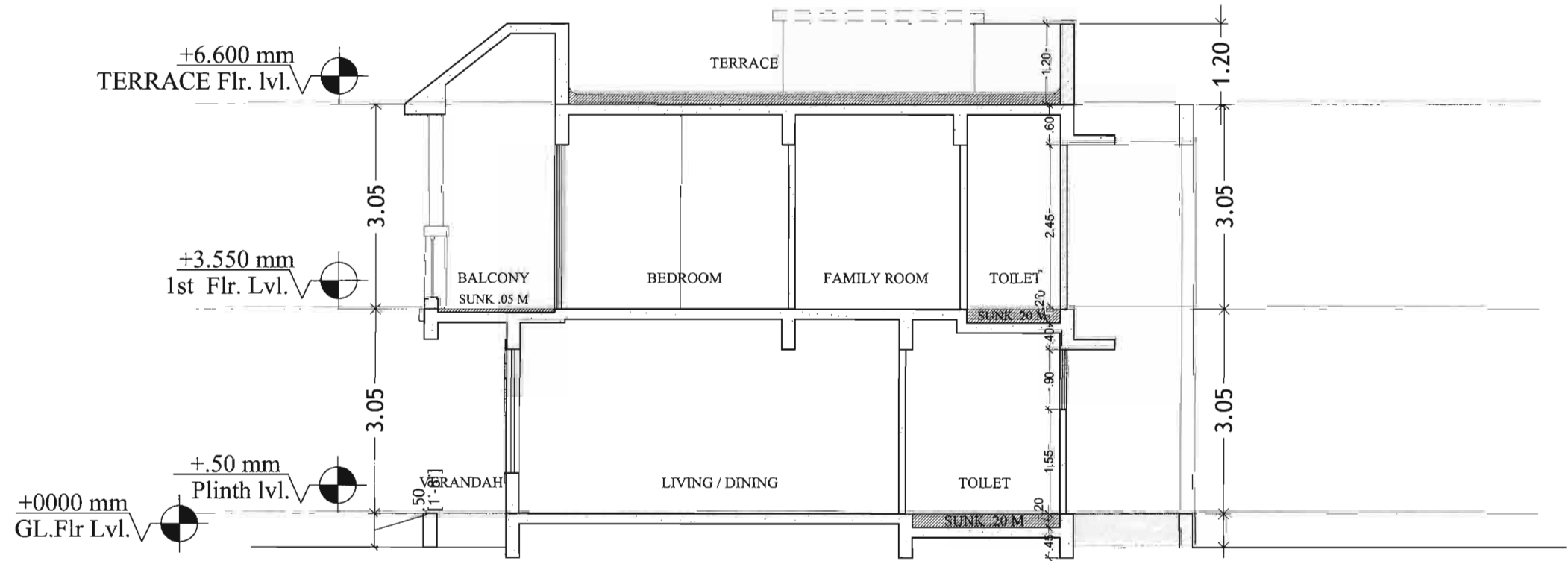
SECTION ON 2-2
