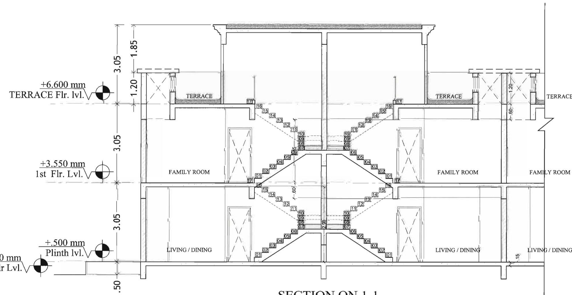
SECTION ON 1-1
