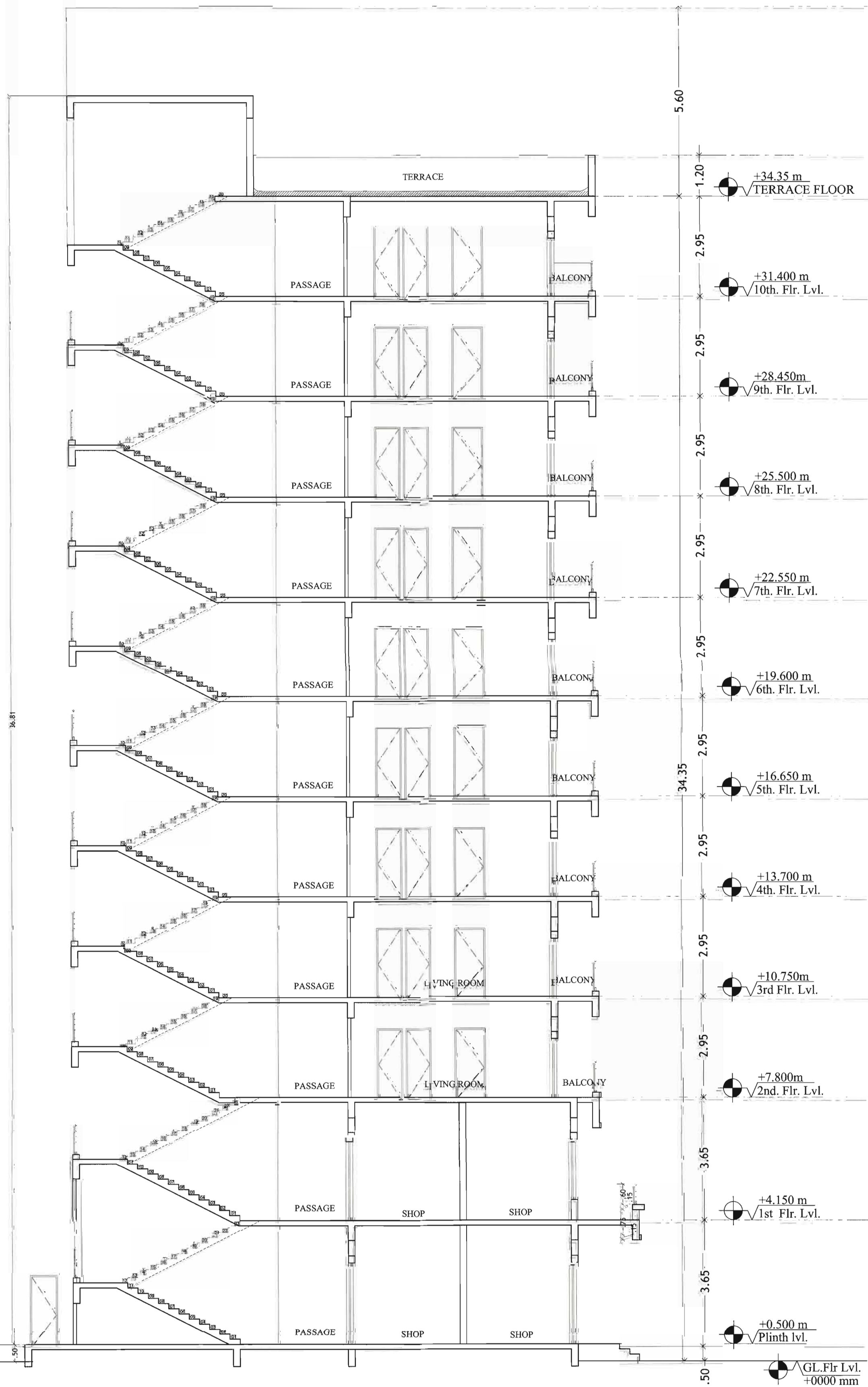
SECTION ON 03-03
